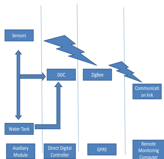
Fig. 1.: Hardware system for precision agriculture irrigation based on the Internet of things
